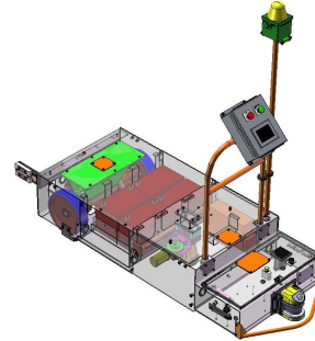
AUTOMATED GUIDED CARTS SHOWN VARY BASED ON CUSTOMER SELECTED OPTIONS
